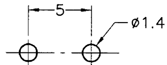
MOUNTING HOLES
