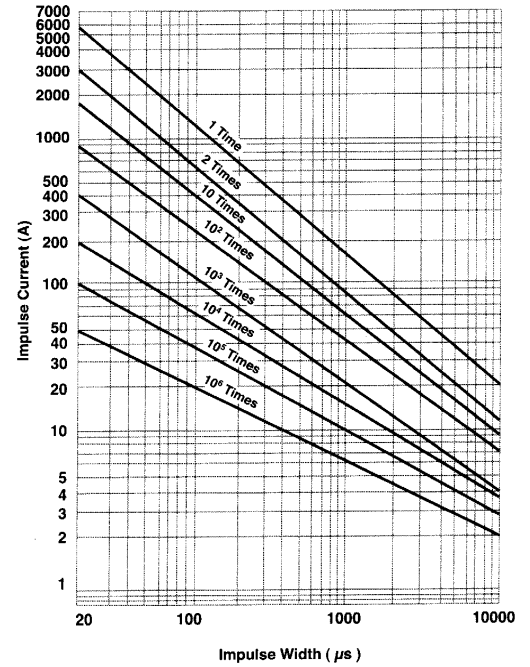
V-I Surge Life Time Ratings (820K to 561K)
