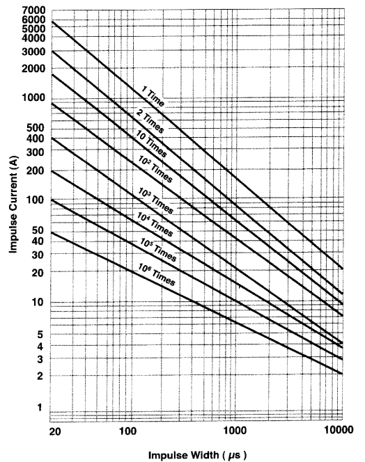
V-I Surge Life Time Ratings (621K to 182K)
