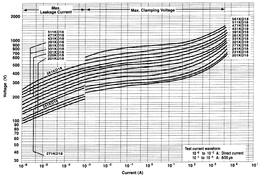
V-I Curve (820K to 561K)
