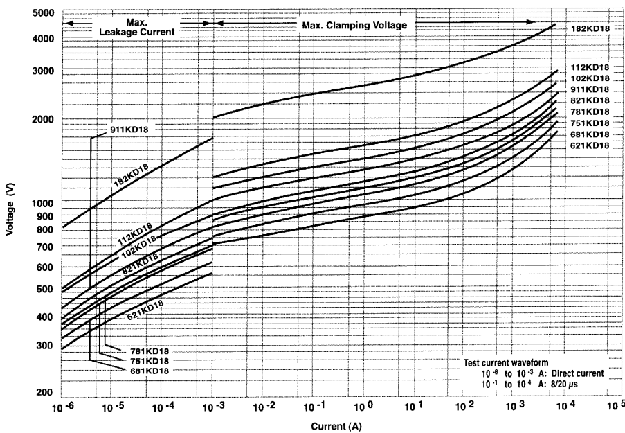
V-I Curve (621K to 182K)
