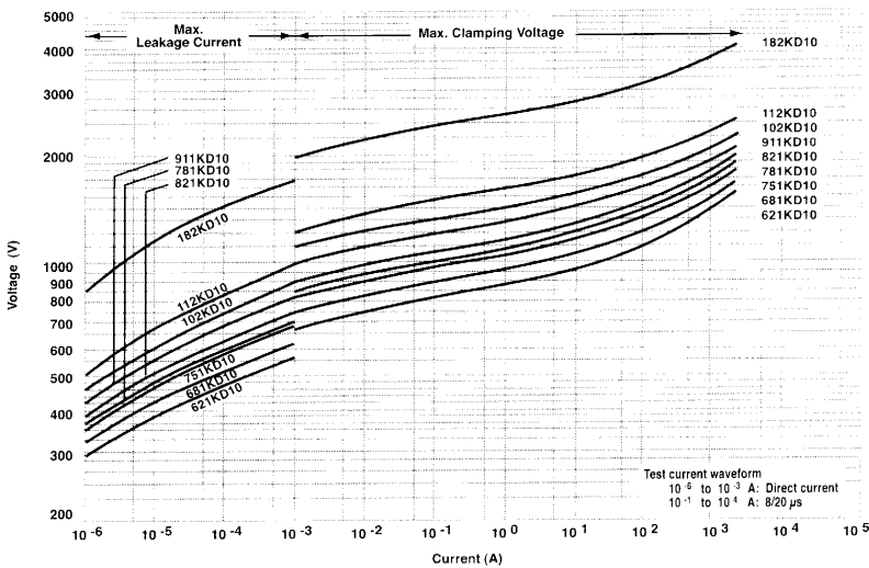
V-I Curve (621K to 182K)
