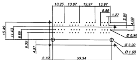
PCB LAYOUT (Top View)
