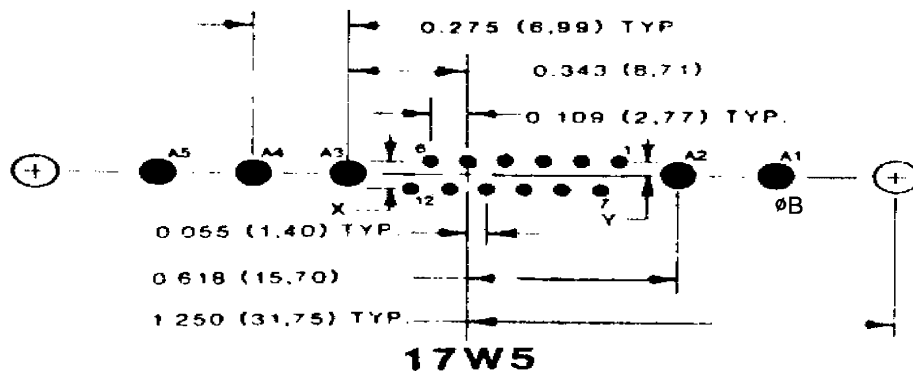
PCB LAYOUT
