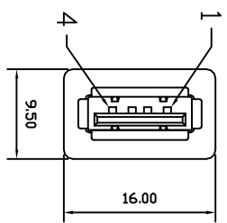
USB A FEMALE
