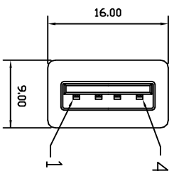
USB A MALE
