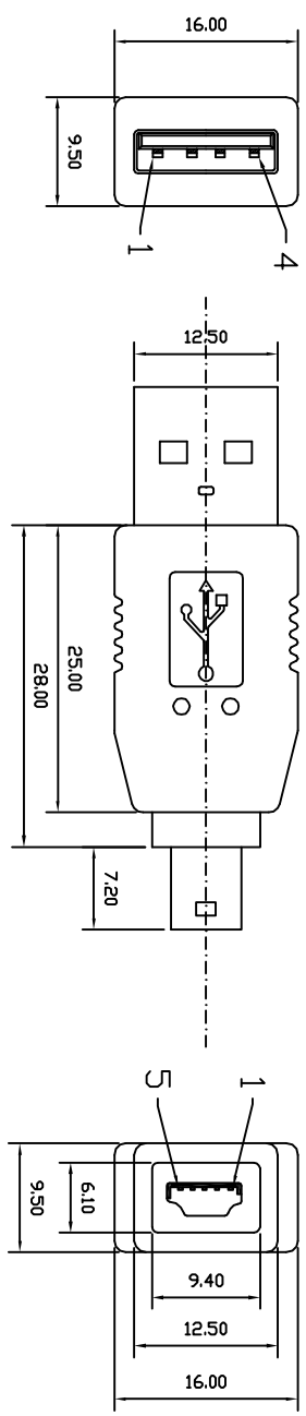
USB A MALE
