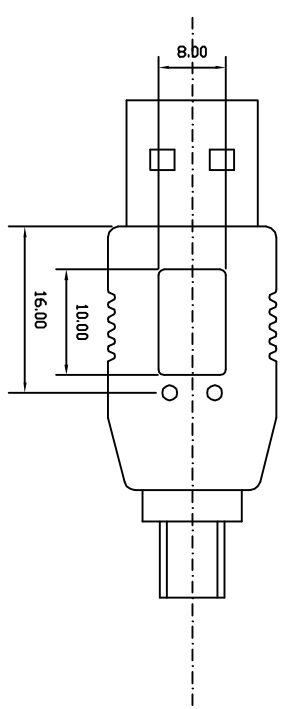
USB-A MALE 1 2 3 4 SHELL
