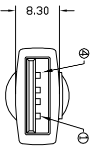
USB-A MALE
