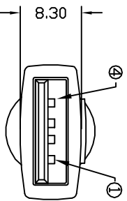
USB-A MALE
