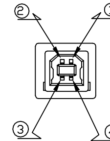
USB-B FEMALE
