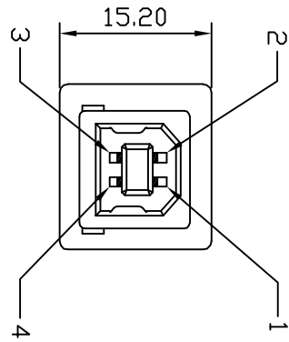
USB-B FEMALE
