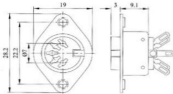
SOLDER TYPE DS-074-DS-078
