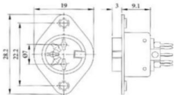
PCB TYPE DS-074-P~DS-078-P
