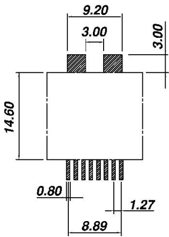
PBC Layout (Top View)
