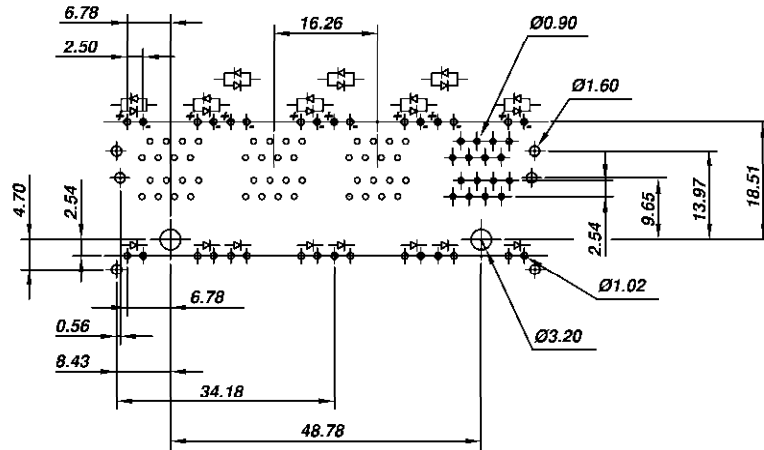
PC Layout (Top View)
