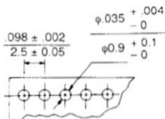
P C. Board Hole Dimensions
