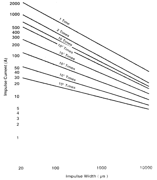
V-I Surge Life Time Ratings (330K to 680K)
