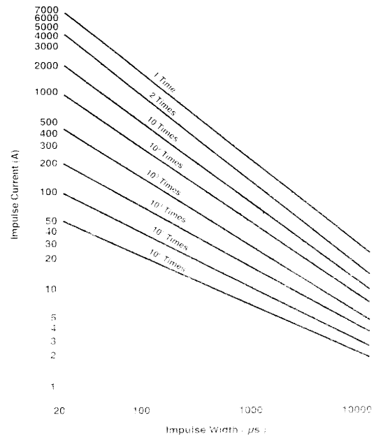
V-I Surge Life Time Ratings (820K to 182K)
